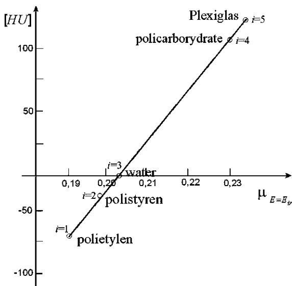
Fig. 9.8 Evaluation of the linearity of a CT scanner
