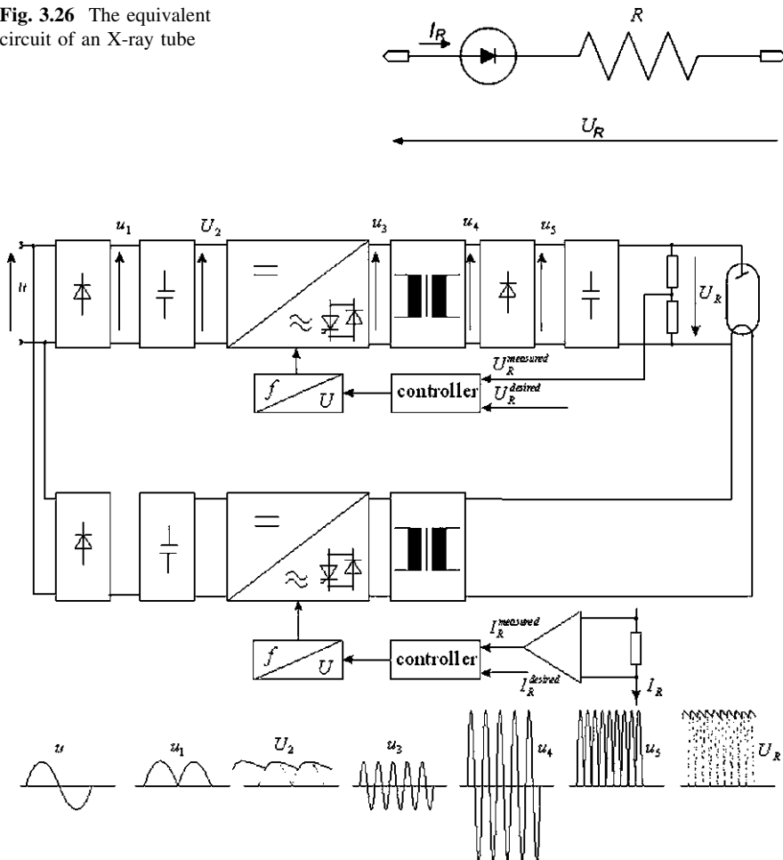
Fig. 3.27 A circuit diagram for an X-ray tube used for medical purposes
