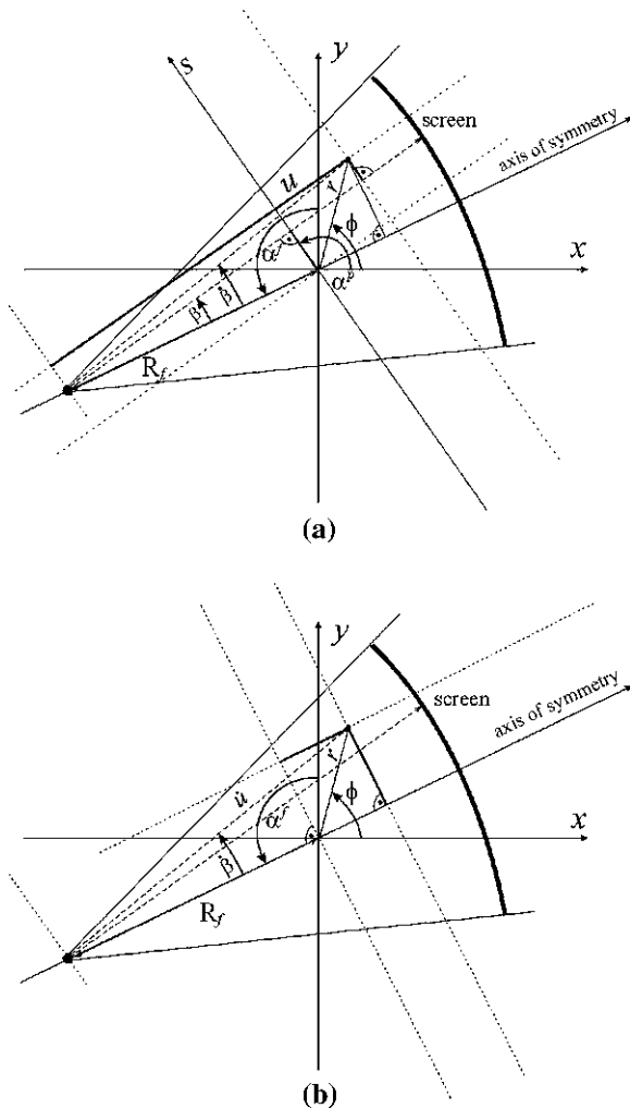
Fig. 6.7 Determination of the polar coordinates of a point in the plane of a fan-beam projection: a derivation of (6.21), b derivation of (6.22) and (6.23)
