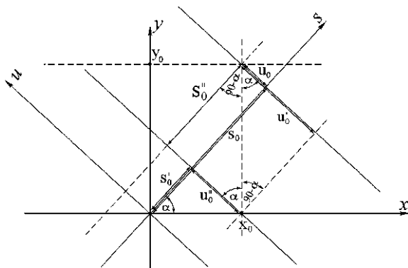
Fig. 4.8 Details of the trigonometric relationships in a parallel-beam scanner
