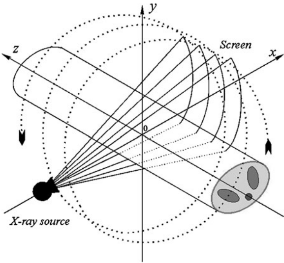
Fig. 7.15 The projection system of a multi-slice spiral scanner—a three-dimensional perspective view
