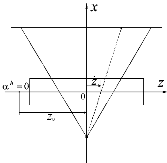
Fig. 7.28 The geometry of the scanner in the x - z plane
