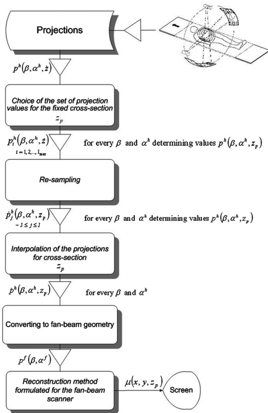
Fig. 7.21 The z -filtering algorithm used in MSCT tomography
