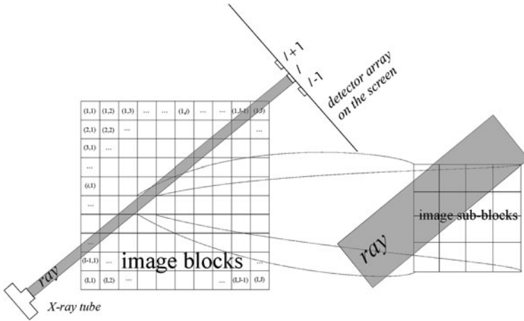
Fig. 8.2 The determination of \chi_{ij}(l, \psi) : a determination of the set of image blocks taking part in the formation of the projection value, b a way of determining the contribution a given image block makes to the formation of a specific projection value
