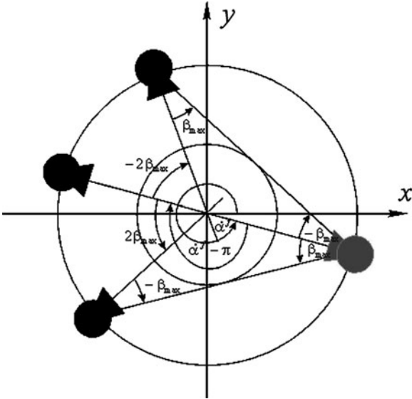
Fig. 7.11 Selecting complementary projection values
