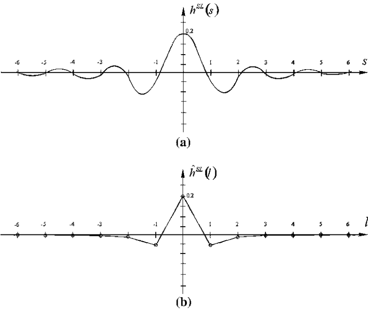
Fig. 5.21 A Shepp–Logan filter in the s -domain: a in the form of a continuous function; b in its discrete form
