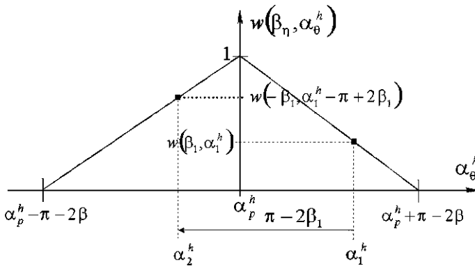
Fig. 7.13 A graph of the weighting function w(\beta_\eta, \alpha_\theta^h) determining the weight assigned to each projection \hat{p}^h(\eta, \theta) in the 180° LI method
