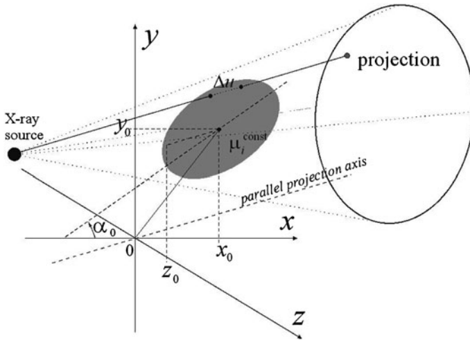
Fig. 10.12 Determining the projection value of an ellipsoid rotated through an angle \alpha_0 and displaced by the vector (x_0, y_0, z_0)
