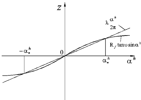
Fig. 7.48 Graphs of R_f \tan v \sin \alpha^h and \lambda \frac{\alpha^h}{2\pi} , assuming the condition in (7.153) is fulfilled
